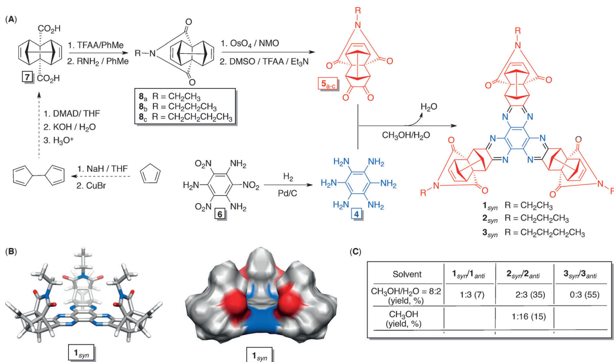
Figure 1. A) The preparation of C 3v symmetric 1 syn –3 syn can be completed on a large scale using simple starting materials and a convergent synthetic strategy. B) Energy-minimized structure of 1 syn (MMFFs, Spartan) and van der Waals surface of this molecule showing its cavity (V = 123 Å 3 ); gray C, red O, blue N. C) The condensation of hexaaminobenzene 4 (in CH 3 OH/H 2 O) and diketone 5 a-c (in CH 2 Cl 2 ) gives syn and anti diastereomers of 1–3 in different ratios (yields are of isolated products).
